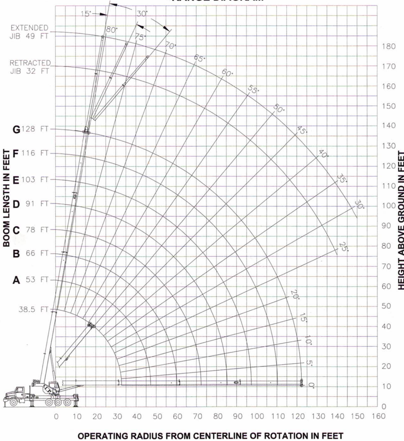
- RANGE DIAGRAM -
